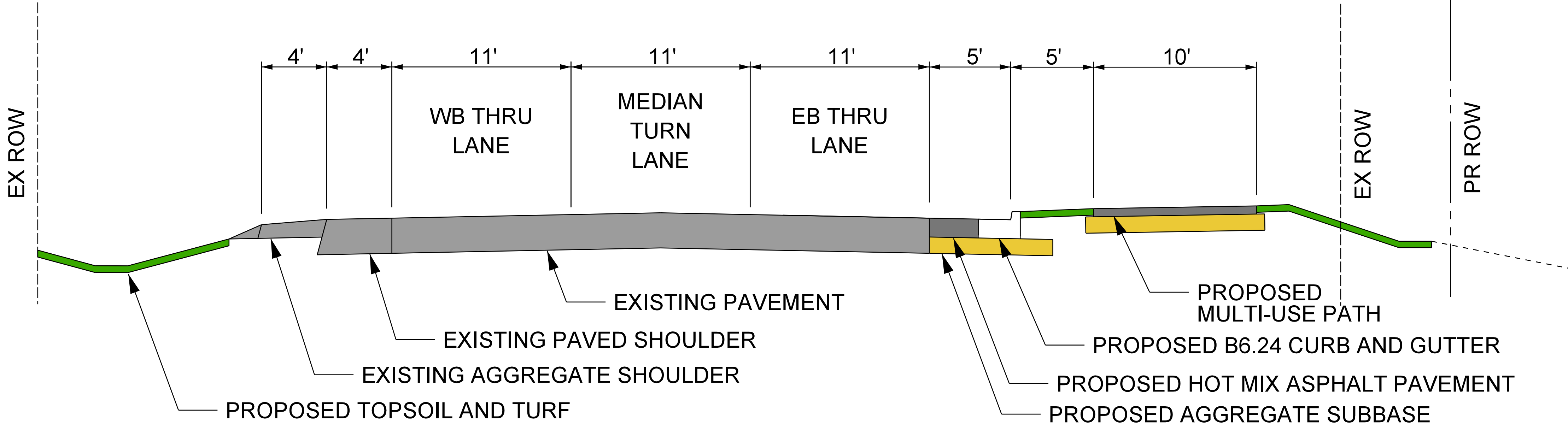
PROPOSED GILMER ROAD MULTI-USE PATH W/ CC&G
